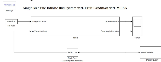
Figure 10: Simulink model for SMIB with MB-PSS
