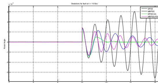
Figure 13: Comparison for rotor angle deviations of different methods for fault at t=10 sec
