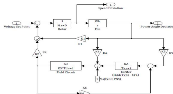
Figure 3: Simulink Implementation of SMIB
