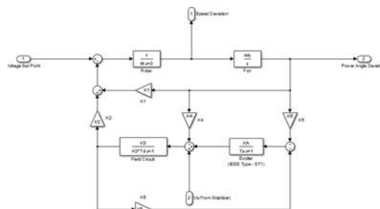
Figure 2: Heffron-Phillips model – SMIB
