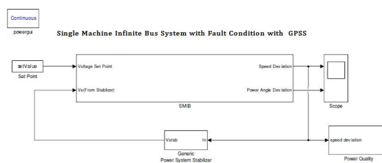
Figure 7: Simulink model for SMIB with GPSS
