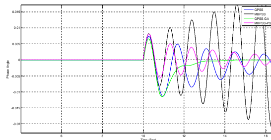
Figure 14: Comparison for phase angle deviations of different methods for fault at t=10 sec
