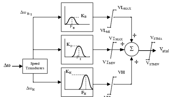
Figure 8: Multi-band power system stabilizer (MB-PSS)
