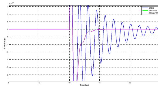
Figure 14: Comparison for phase angle deviations of GPSS, GPSS-GA and GPSS-PSO methods for fault at t=10 sec
