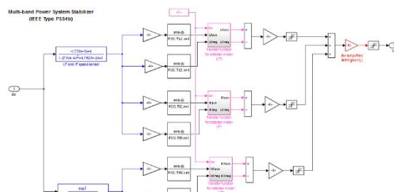
Figure 9: Simulink model for MB-PSS
