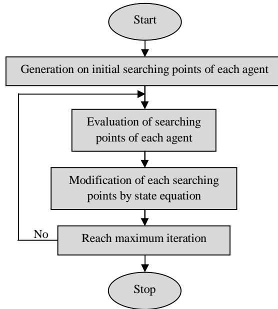
Figure 12: Flow chart of PSO algorithm
